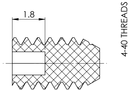
SECTION X-X
